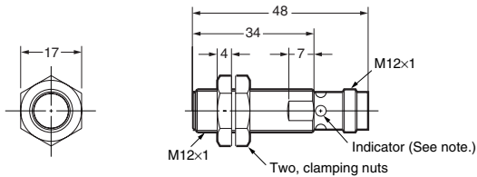
E2A-M12KS04-M1-□□/E2A-S12KS04-M1-□
